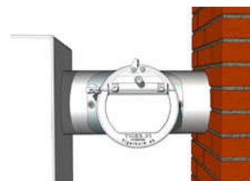
Tigex 25 with integrated adapter (60390/100E) for round flue pipe Ø100 mm
